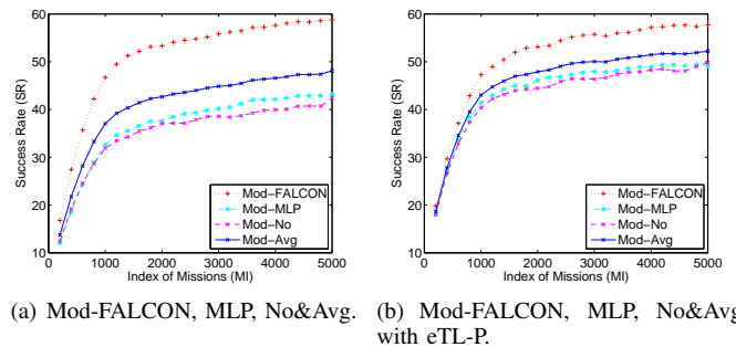
Fig. 9. SRs of Mod-FALCON, Mod-MLP, Mod-No and Mod-Avg on completing the missions in PO-MNTs.
