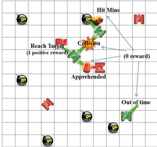
Fig. 3. An illustration of the adapted MNT (PO-MNT).
