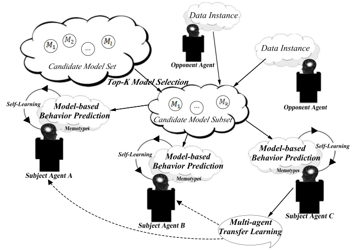
Fig. 2. An illustration of the proposed eTL-P.
