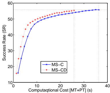
Fig. 8. SRs of MS-C and MS-CD over computational cost ((MT+PT)) on completing the missions in PO-MNTs.
