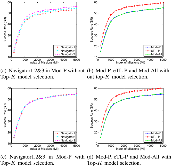
Fig. 7. SRs of navigators with 99 predictive candidate models on completing the missions in PO-MNTs.
