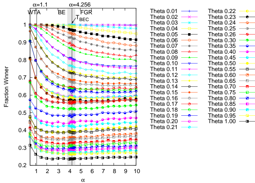
Fig. 4. Fraction Winner of 3-SAT. We report the number of links shared by the winner node against \alpha . After a decrease for low values of \alpha , the FW is almost linear for high values of \theta . For low values of \theta , we observe a nonlinear variation, meaning that if \alpha approaches 0, the number of BEC cases increases with a high derivative. This behavior of \theta is strongly related to the physical property of having a large number of BECs when the absolute temperature approaches 0.
