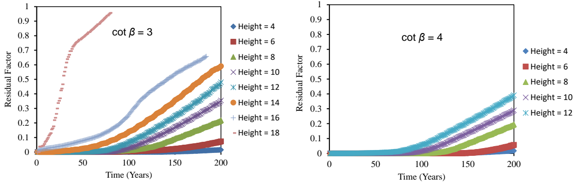
Figure 4: Residual factor with time
