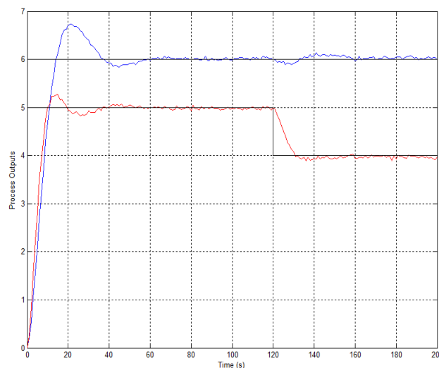
Fig. 7 Simulation results for SPC_2 controller with \lambda = [0.4, 2] .
