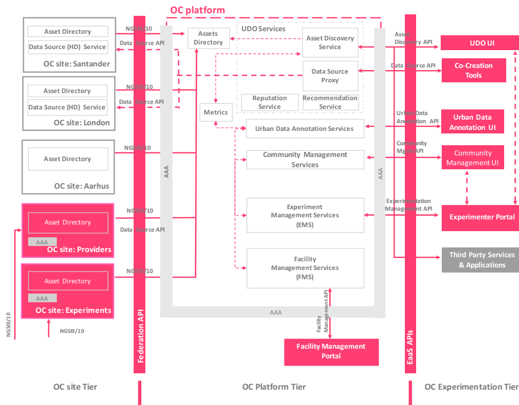
Figure 2. OrganiCity EaaS facility architecture instantiation.
