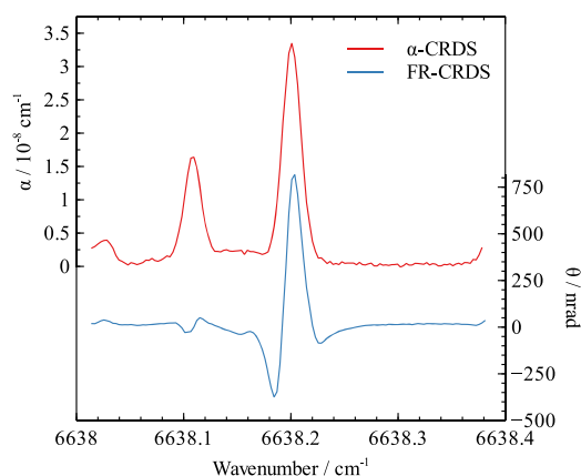
FIG. 2. Absorption and Faraday rotation spectra of \text{HO}_2 around 6638.2\text{ cm}^{-1} at 30 Torr ( B = 694\text{ G} ). The spectra cover both the {}^q\text{Q}_3(N = 4-9) transitions ( 6638.20\text{ cm}^{-1} ) and {}^q\text{P}_0(6) transition ( 6638.11\text{ cm}^{-1} ).
